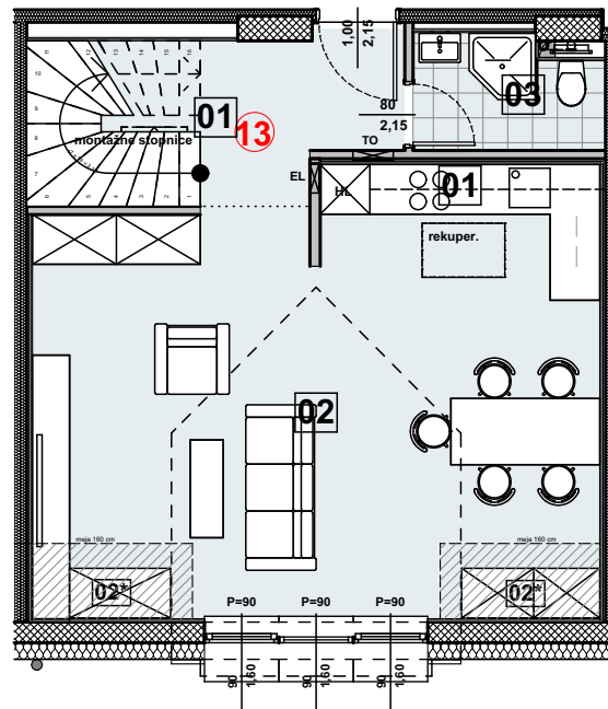
1 MANSARDA 1 1:100
