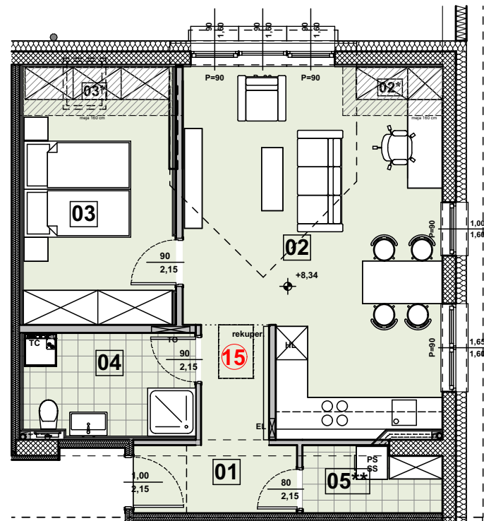
MANSARDA 1
