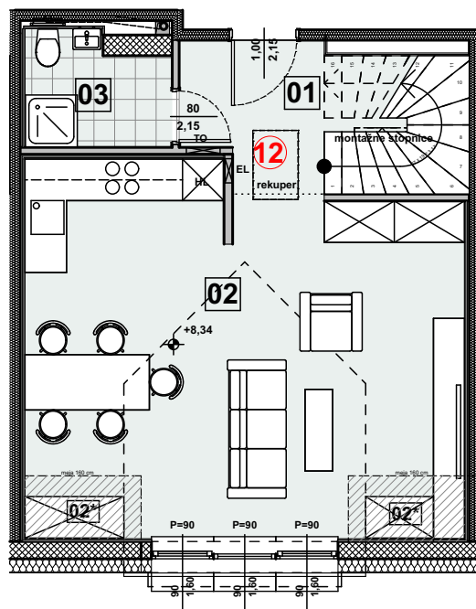
1 MANSARDA 1 1:100
