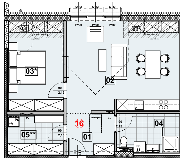
MANSARDA 1
