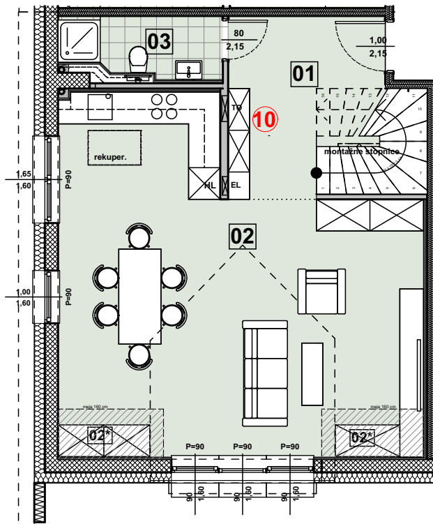
1 MANSARDA 1 1:100
