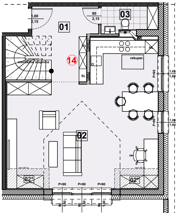
1 MANSARDA 1 1:100
